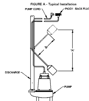
Dimensions: A=9' B=3.42 C=2.81
