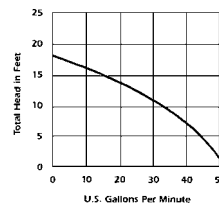
PERFORMANCE CURVE
